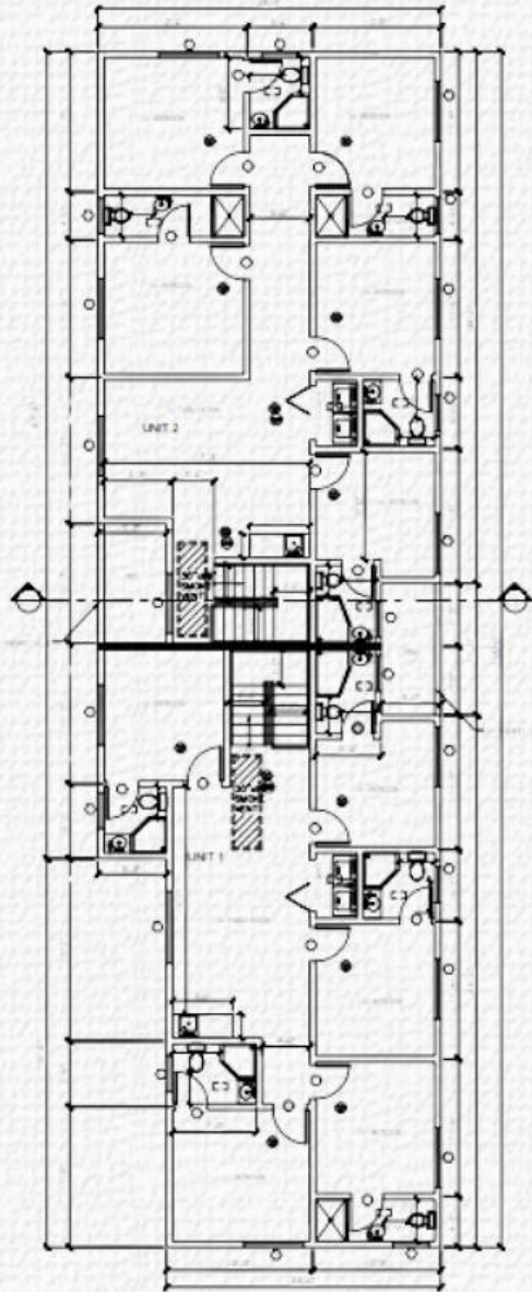
Third Floor
